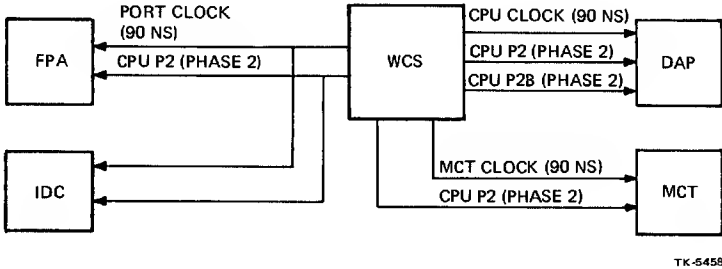
Figure 3-1 Clock Distribution
